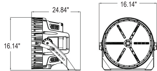
Flood Mount
