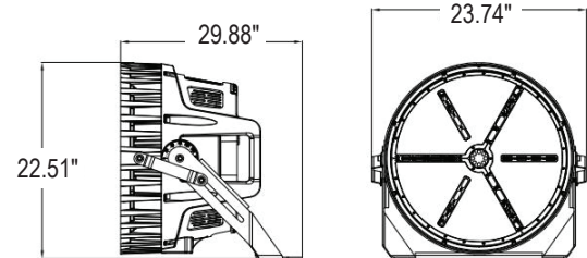
Flood Mount
