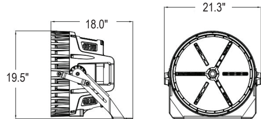
Flood Mount
