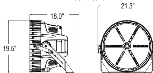
Flood Mount
