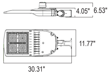
Yoke Mount
