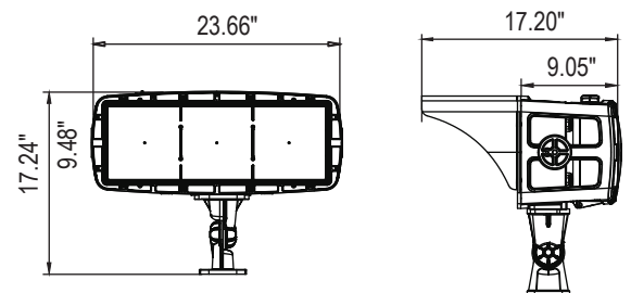
Yoke Mounting Bracket
