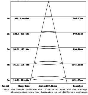
Flux out: 3450 lm
